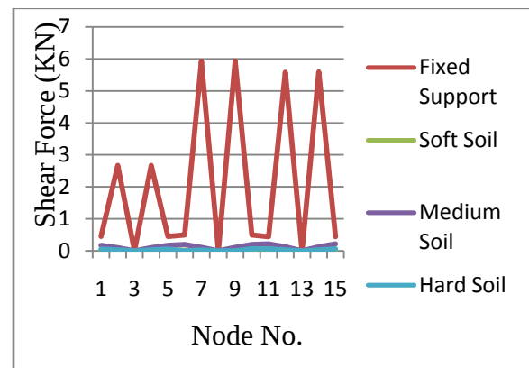
Fig. 5.4 Shear force of Fixed Support and Fixed but Support
