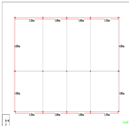
Fig. 4.1 Plan of R.C.C. Frame Structure
