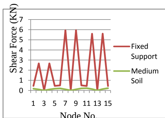
Fig. 5.2 Shear force of Fixed Support and Medium Soil
