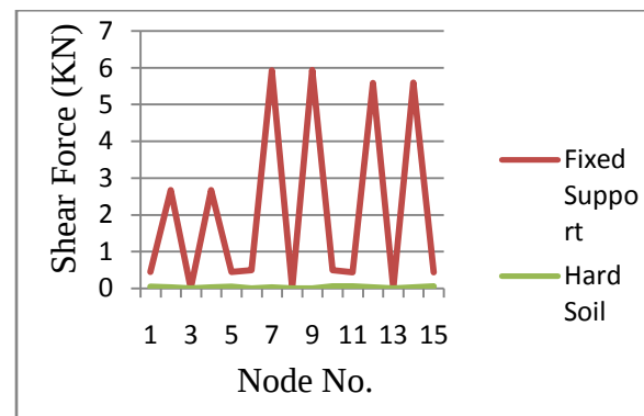
Fig. 5.3 Shear force of Fixed Support and Hard Soil
