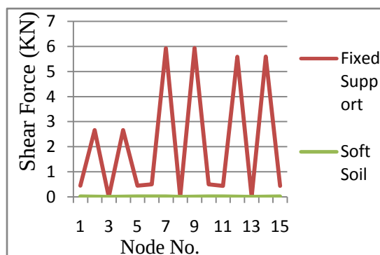
Fig. 5.1 Shear force of Fixed Support and Soft Soil
