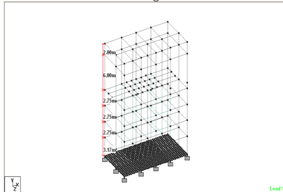
Fig. 4.2 3D View of R.C.C. Frame Building
